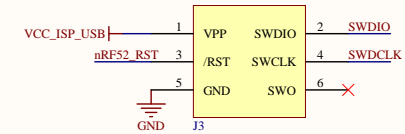
JTAG connector for ISP4520 programming via JTAG Interface
